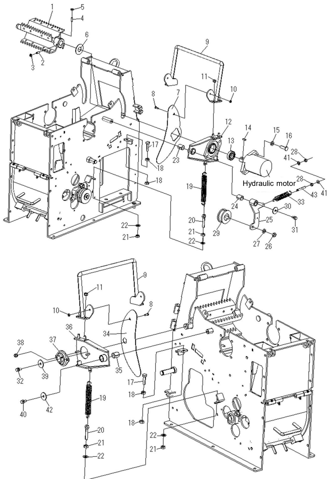
Fig. 11 Feeding system
