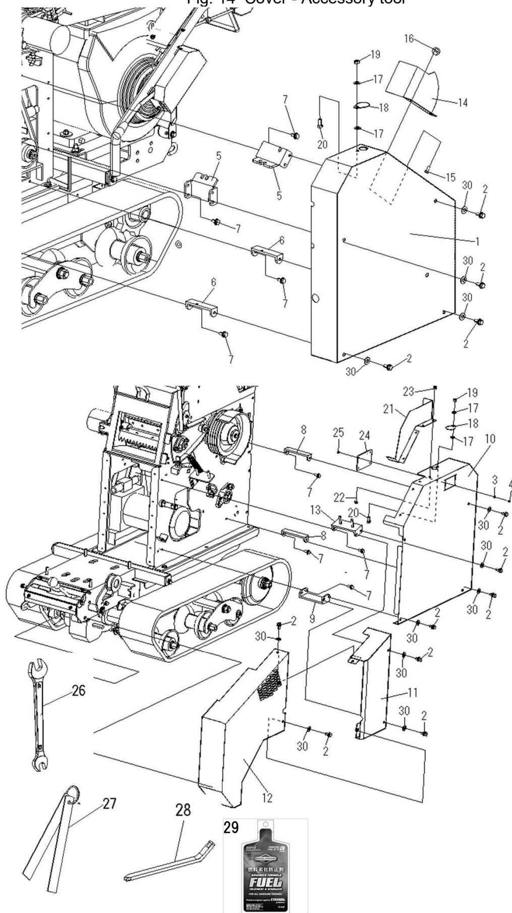
Fig. 14 Cover - Accessory tool
