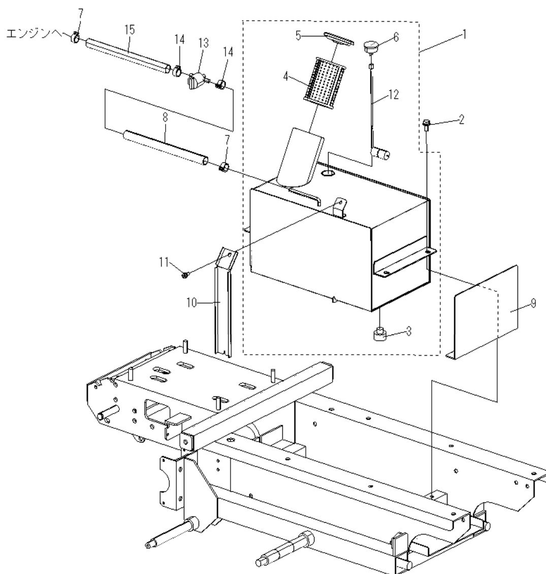
Fig. 5 Fuel tank
